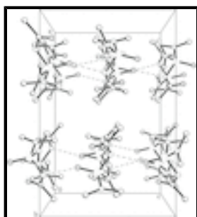
Fig. 2. A projection of packing diagram of the title compound along the y direction. Hydrogen bonds are indicated by dashed lines. H and Cl atoms are omitted for clarity.
