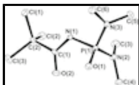
Fig. 1. Structural representation of 1 with atom numbering scheme and 50% probability thermal ellipsoid. The hydrogen atoms are omitted for clarity.
